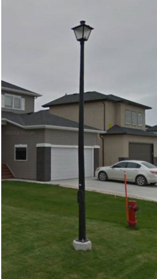
15' COLONIAL POST TOP, BLACK GALVANIZED STANDARD, CONCRETE FOUNDATION
