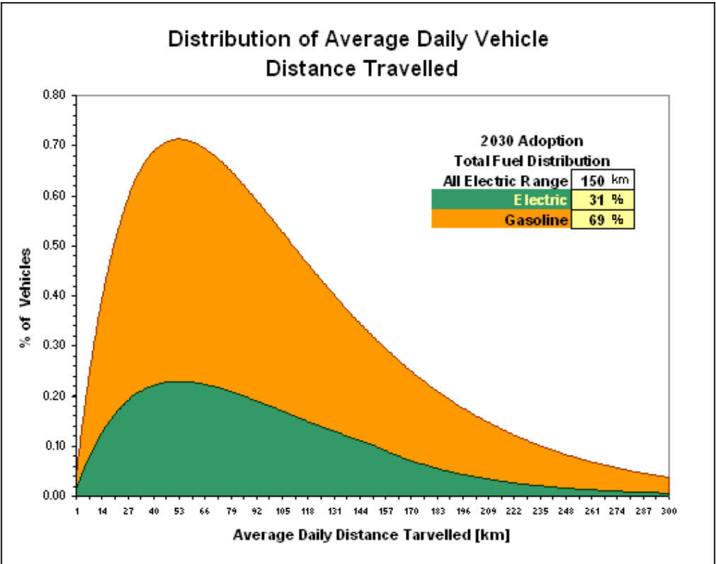
Figure 7: 2030 PDF of Daily Vehicle Average Distance Travelled with 150 km PEV Net-Electric Range (Medium Adoption Scenario for Manitoba)
